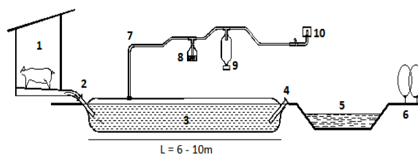
Figure 3. The PE digester 1 - Pig-pen; 2 - Inlet pipe; 3 - Digester; 4 - Outlet pipe; 5 - Discharge pond; 6 - Garden; 7 - Gas vent; 8 - Security valve; 9 - PE gas-holder; 10 - Stove (Author: Vo, H. N.)
