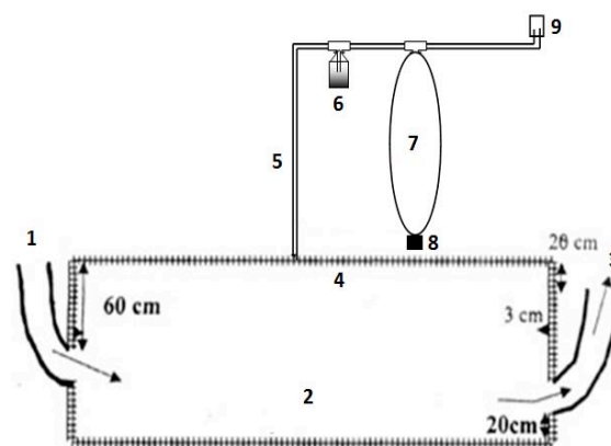
Figure 15. The improved rectangular parallelepiped biogas plant
