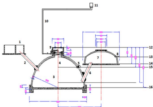
Figure 5. The sketch of TG-BP biogas plant 1 - Inlet tank; 2 - Inlet pipe; 3 - Digester; 4 - Fixed-dome gas-holder; 5 - Safety belts system; 6 - Outlet pipe; 7 - Compensating tank; 8 - Discharge pipe; 9 - Entry hose with gas-light seal; 10 - Gas pipe; 11 - Stove; 12 - Digester top level; 13 - Ground level; 14 - Zero line; 15 - Security belts level; 16 - Digester bottom level (Source: modified from CENREs, 2002)
