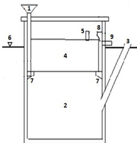
Figure 2. The CT1 biogas plant 1 - Inlet pipe; 2 - Digester; 3 - Outlet pipe; 4 - Gas-holder; 5 - Gas vent; 6 - Ground level; 7 - Gas-holder ring; 8 - Gas-holder stop; 9 - Discharge pipe (Source: Le, 2005)
