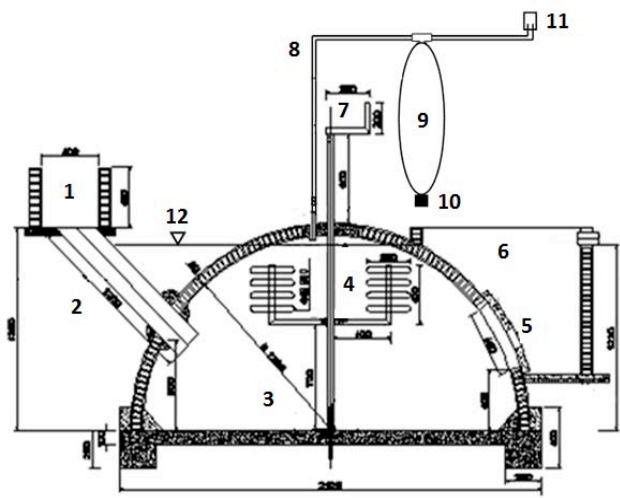
Figure 10. The EQ2 biogas plant
