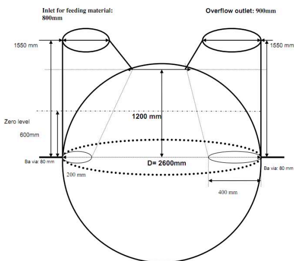
Figure 13. The composite plant (Source: SEDDC, 2010)
