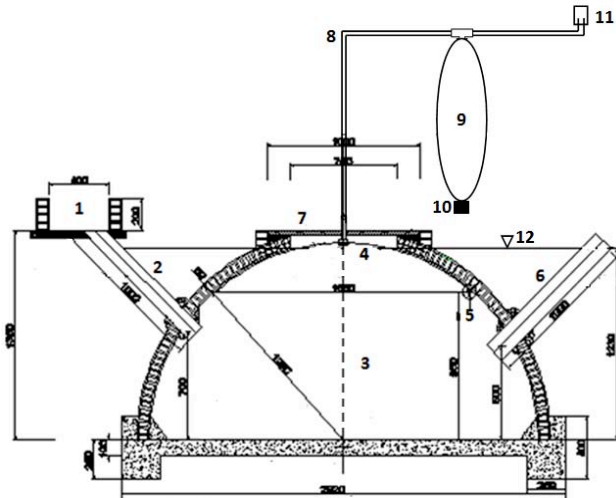
Figure 9. The EQ1 biogas plant
