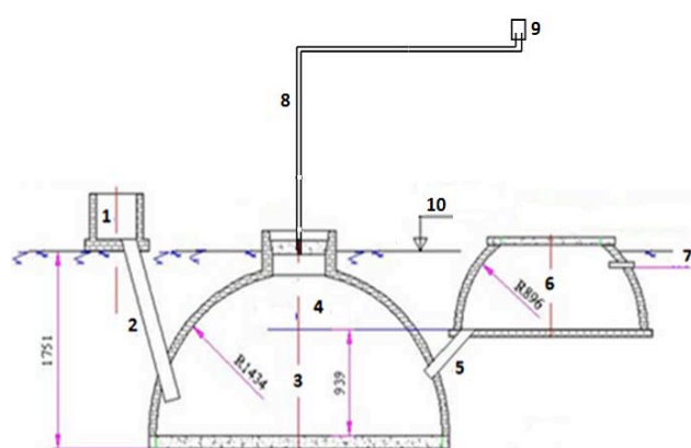
Figure 8. The KT2 domestic biogas plant 1 - Inlet tank; 2 - Inlet pipe; 3 - Digester; 4 - Fixed-dome gas holder; 5 - Outlet pipe; 6 - Compensating tank; 7 - Over-flow level; 8 - Gas pipe; 9 - Stove; 10 - Ground level (Source: modified from Biogas project division, 2008)
