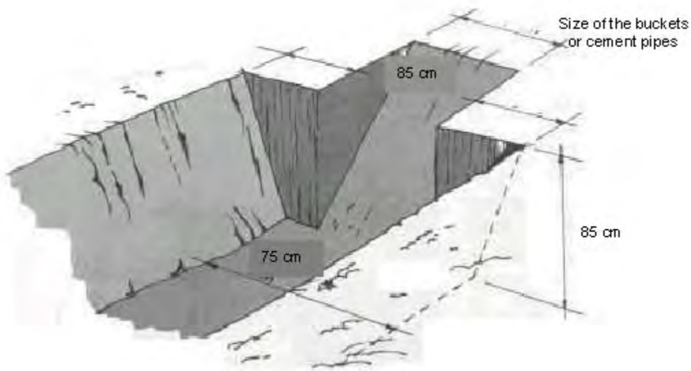
Figure 4. Details of the dug that should be dug at each end of the grave. Source. Botero et al. , 1999.
